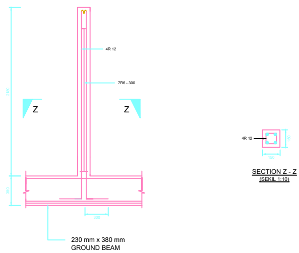
DETAILS OF STIFFENER
