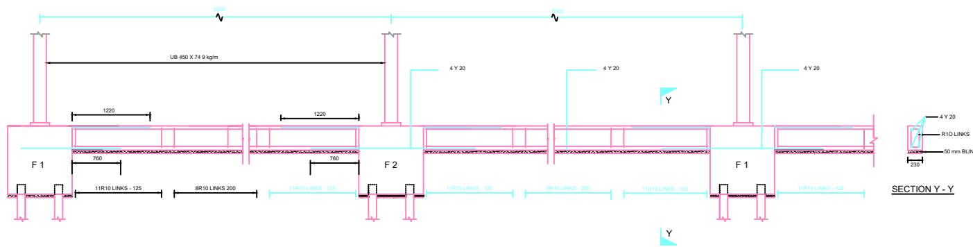
TYPICAL GROUND BEAMS BETWEEN FOUNDATION F1 EXCLUDING ENTRANCE GROUND BEAMS
