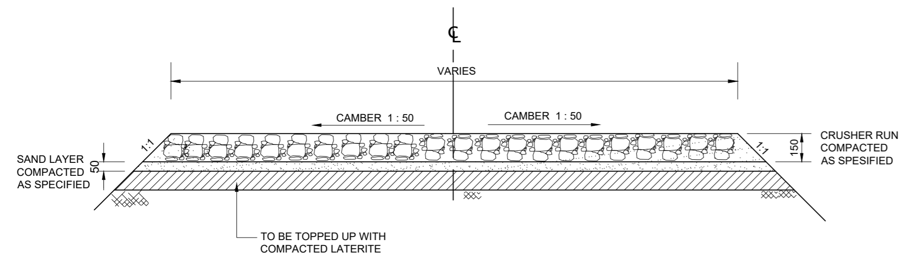
TYPICAL CROSS SECTION OF PROPOSED FARM ROAD
